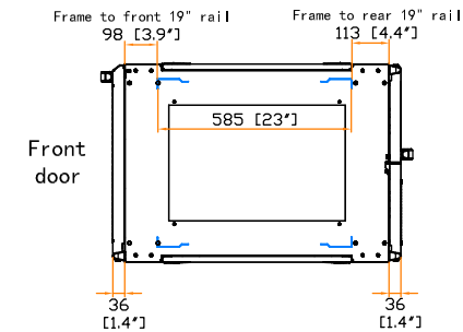
19" rail position
