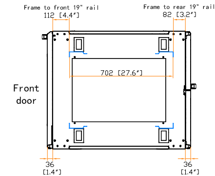
19" rail position
