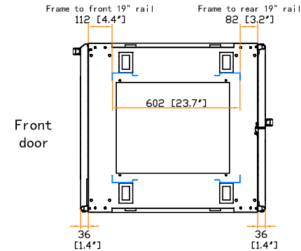
19" rail position
