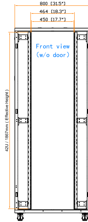
19" rail position
